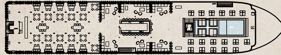
SUNDECK
